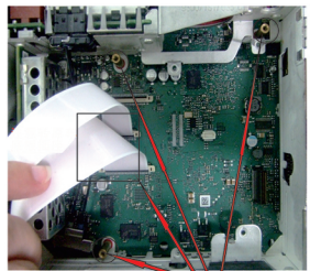
3, unscrew thess three screws, and install three copper post. and then convert well with 2 FPC cable(30P/50P).
